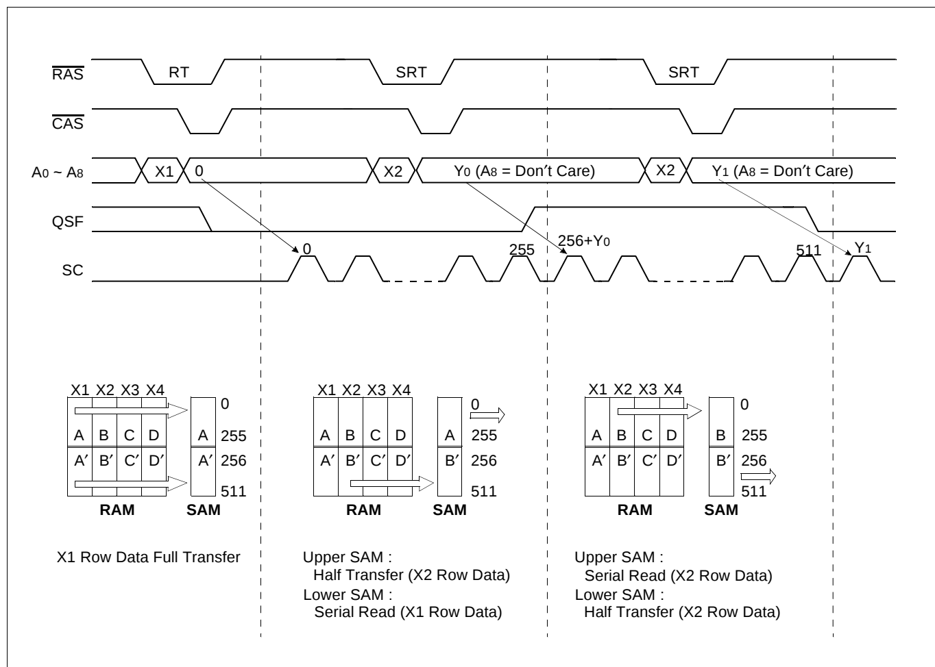
Figure 7. Split Read Transfer Normal Usage
