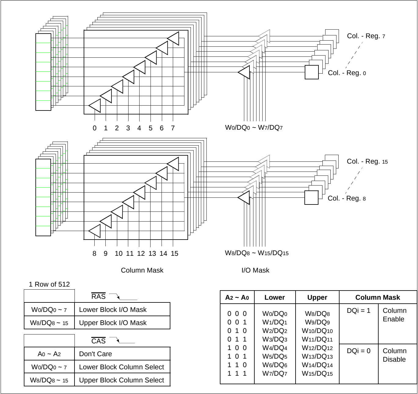
Figure 5. Block Write Scheme
